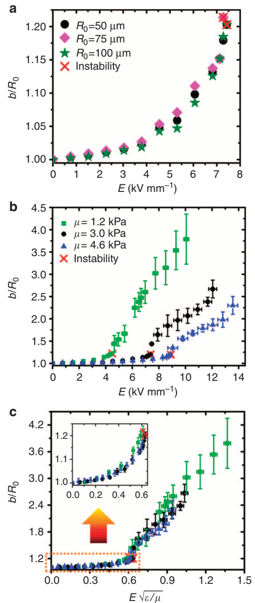
Figure 2 | Deformation and instability of a single drop of conductive liquid in a dielectric polymer under electric fields. The length of the drop is recorded as a function of the applied electric field. The onset of the first sharp tip is marked by a cross. (a) The curves coincide for drops with different radii ranging from \sim 50 to \sim 100 \mu\text{m} in the same polymer. (b) The curves separate for drops in polymers with different moduli (1.2 to 4.6 kPa). (c) The curves for drops in polymers of different moduli coincide again when the electric field is normalized with \sqrt{\mu/\epsilon} . The same markers in b and c indicate polymers with the same \mu . Values in b and c represent mean and s.d. of b/R_0 ( n = 3-4 ).
